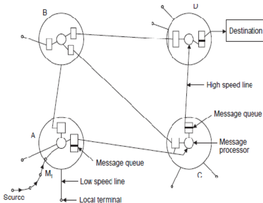
Fig.43: Message switching network.[1]
