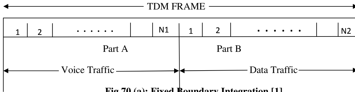
Fig.70 (a): Fixed Boundary Integration [1]
