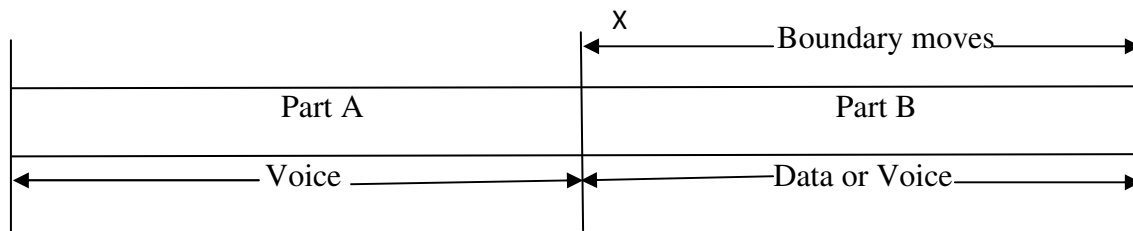
(b) Strategy 2
