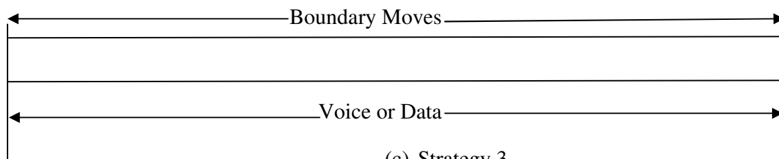
(c) Strategy 3
