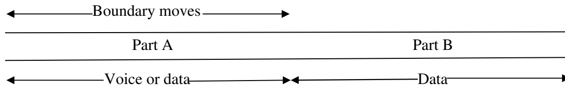
(a) Strategy 1
