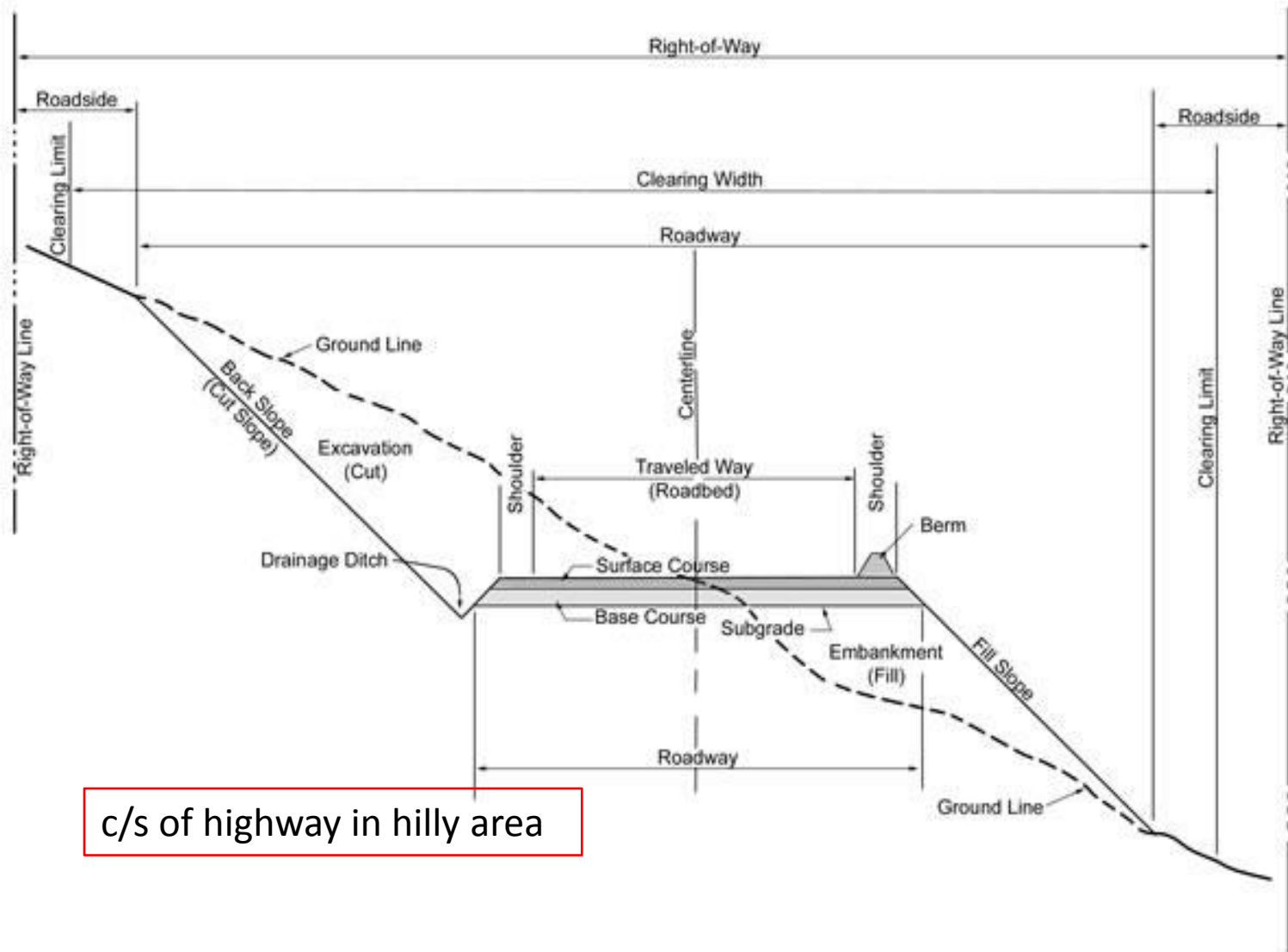
Typical Road Section
