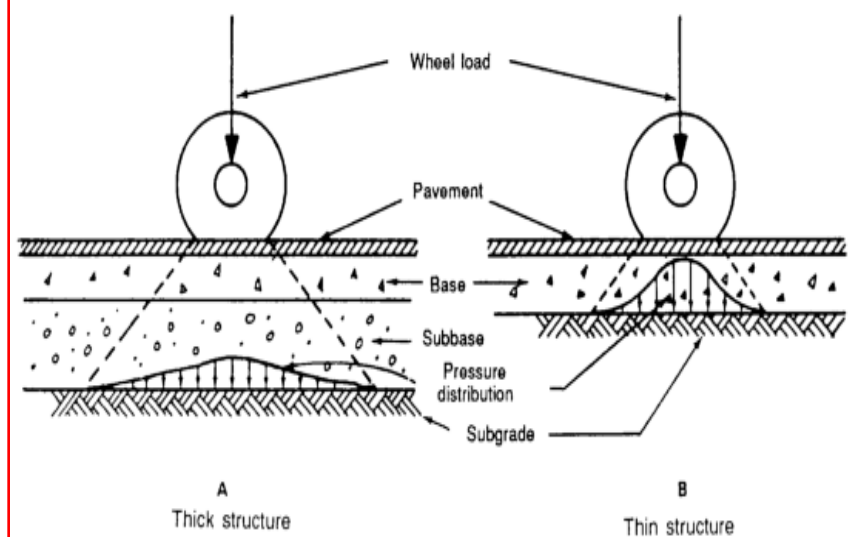
Figure 5-2. Distribution of pressures under single-wheel loads
