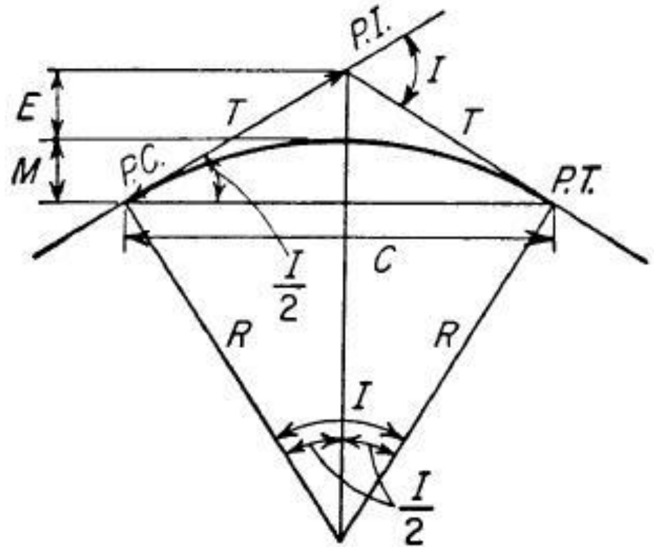
Circular curve.
